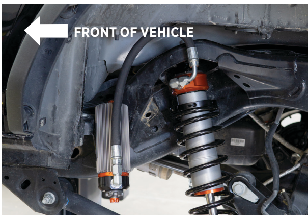
Fig. 39: Face the hose fitting outboard.
