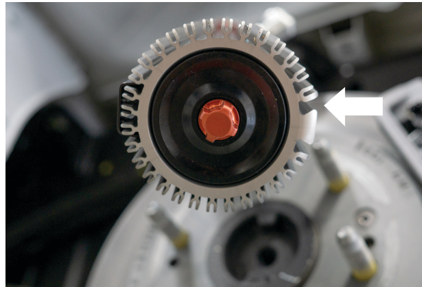
Fig. 21: Lower dovetail marries to the reservoir bracket.
