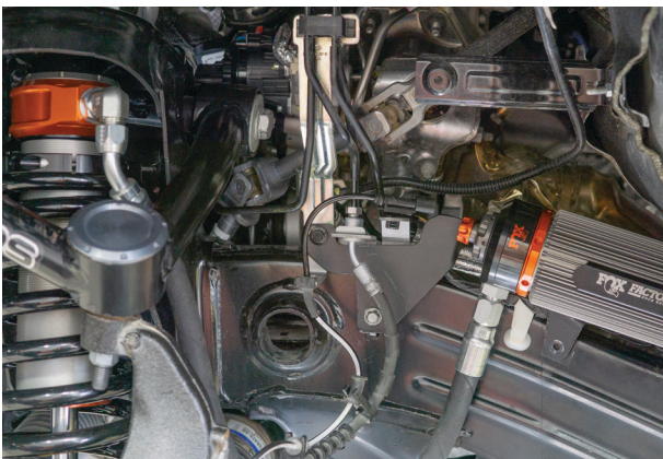
Fig. 26: Mount the reservoir bracket.
