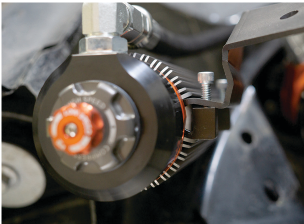
Fig. 42: Mount the reservoir bracket.
