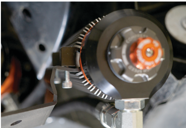
Fig. 22: Mount the reservoir bracket.
