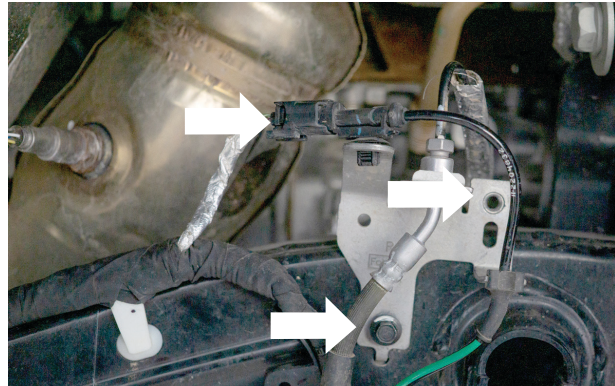
Fig. 24: Disconnect the ABS wire and remove the brake line bracket bolts.
