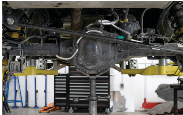
Fig. 35: Support the differential.
